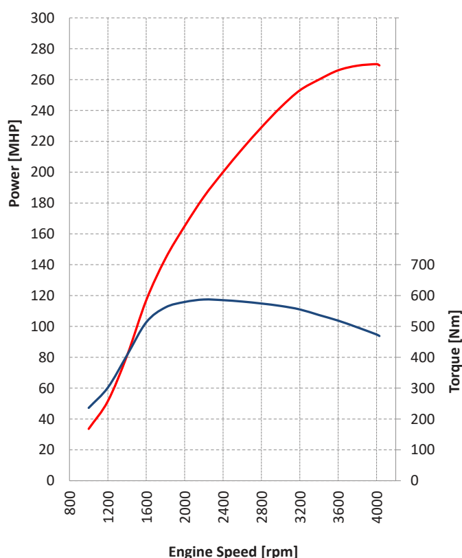
POWER CURVE
